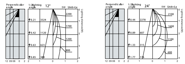
Accurate light distribution and control
