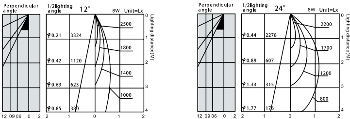
Accurate light distribution and control
